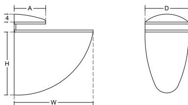
PCA-HR09 Self Holder 5-10mm | Glass Thickness Zinc Alloy | Material Satin, Polished | Finish
