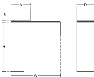
PCA-HR18 Self Holder 5-10mm | Glass Thickness Zinc Alloy | Material Satin, Polished | Finish
